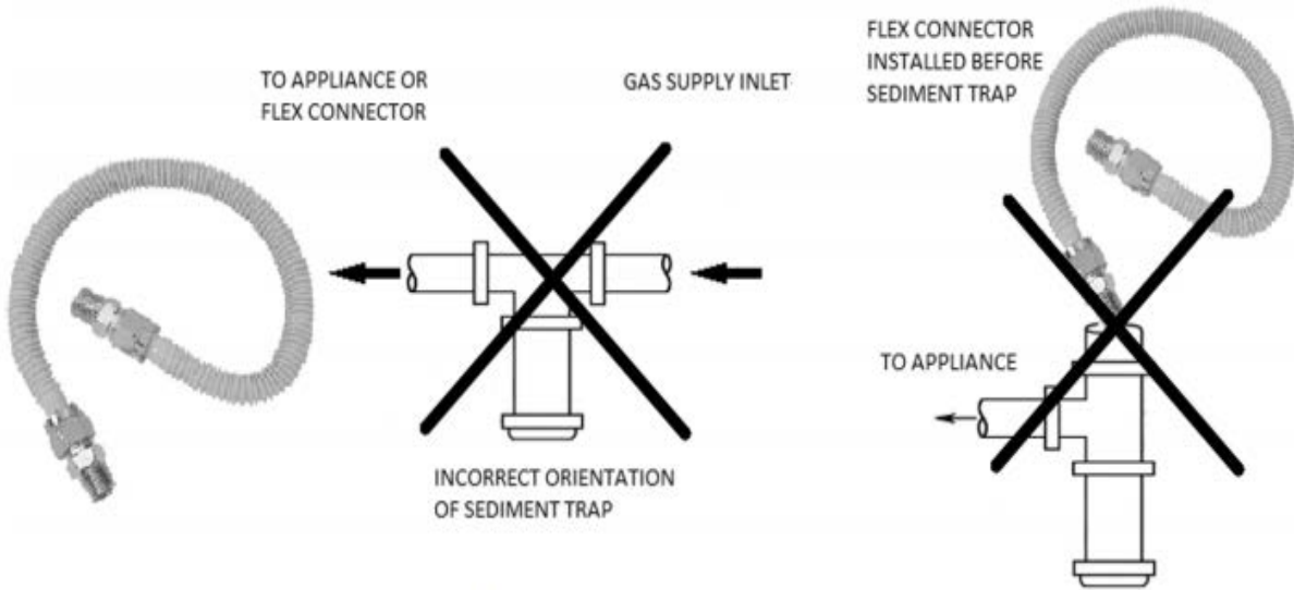
Figure CPA 065 – Improper Installations of Sediment Trap
